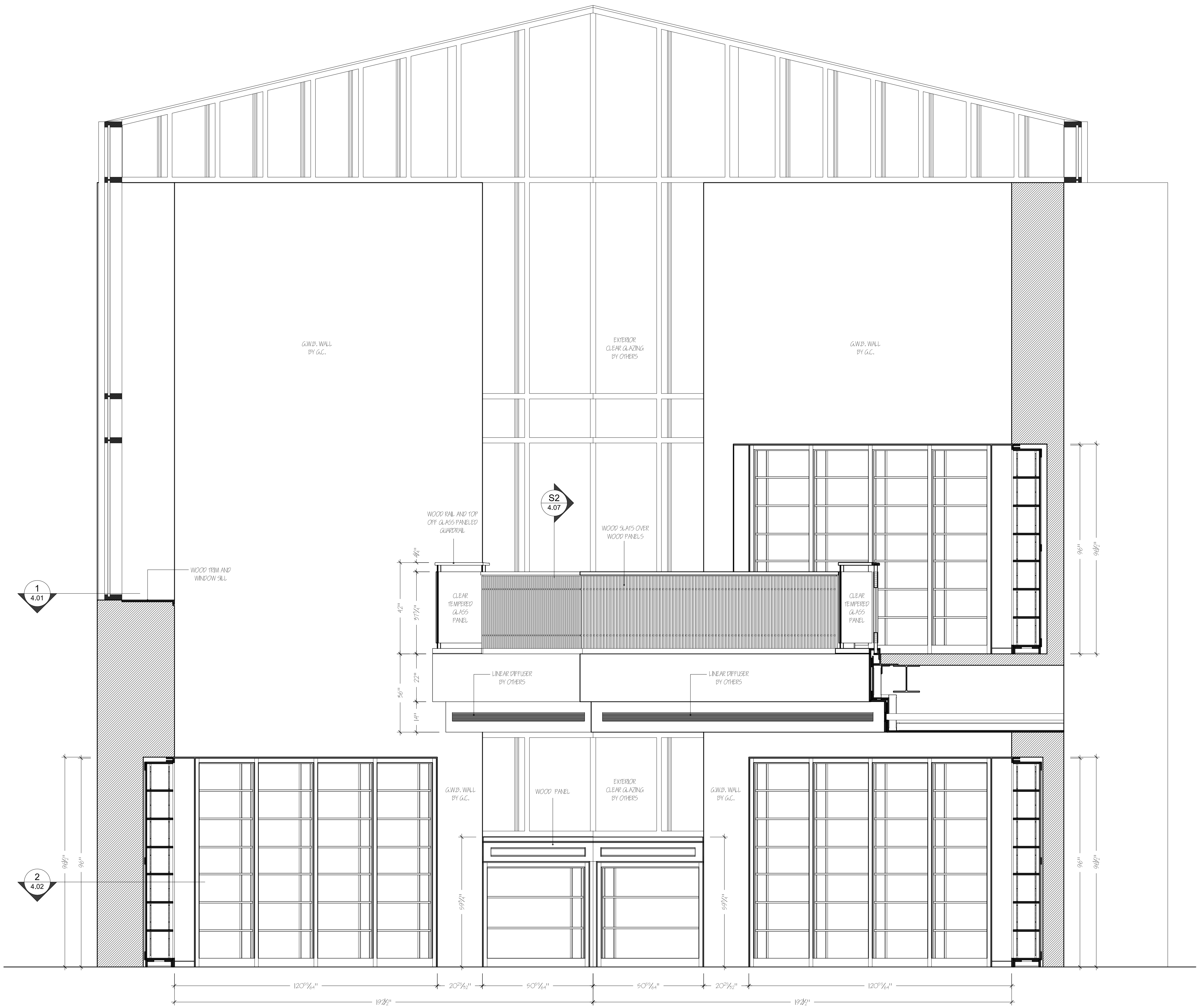
D ELEVATION READING ROOM SCALE: 1/2" = 1'- 0"
