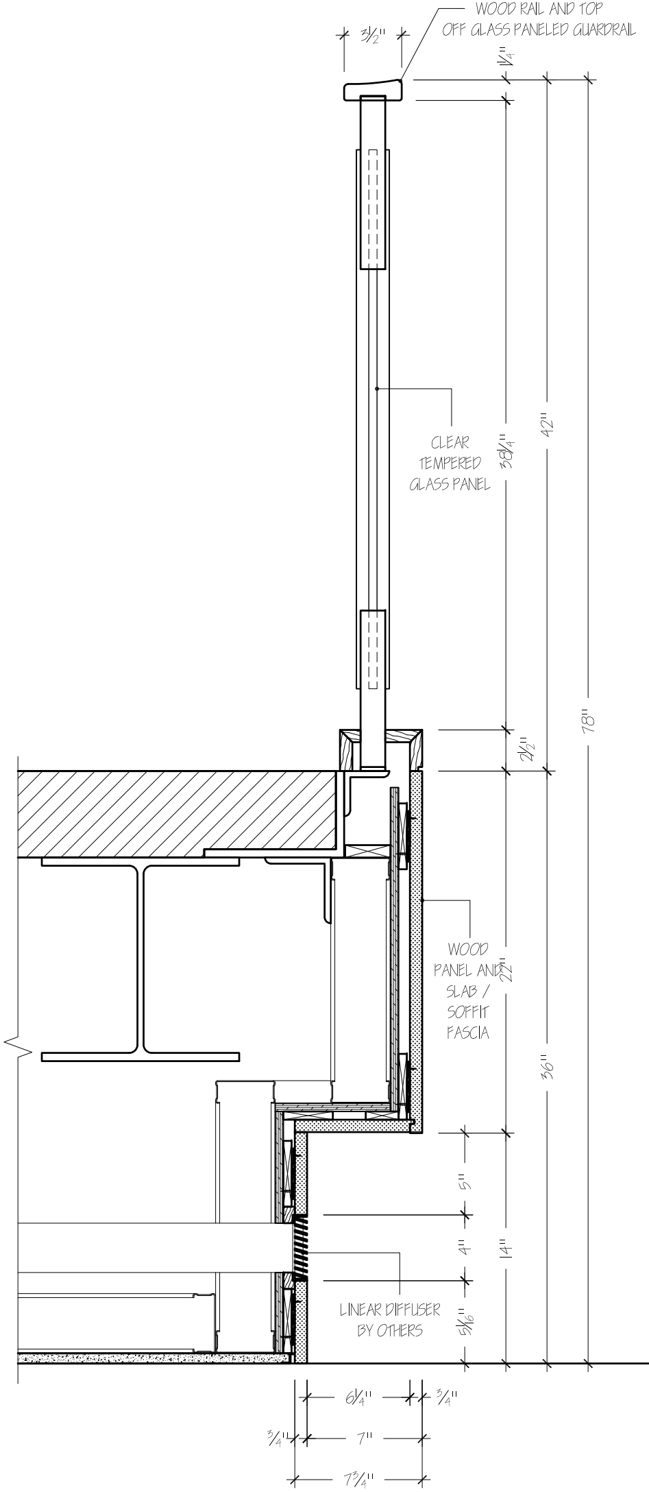
S3 TYPICAL SECTION READING ROOM SCALE: 1-1/2"=1'-0"
