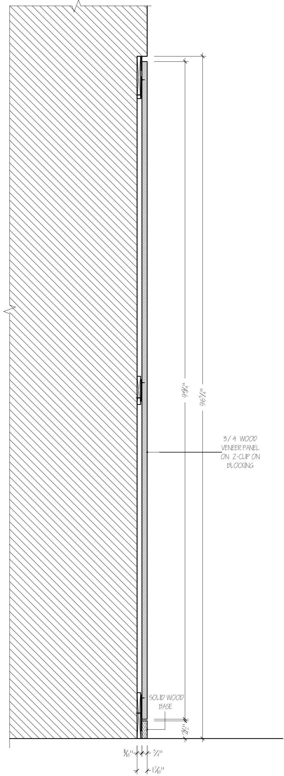
S4 TYPICAL SECTION READING ROOM SCALE: 1-1/2"=1'-0"
