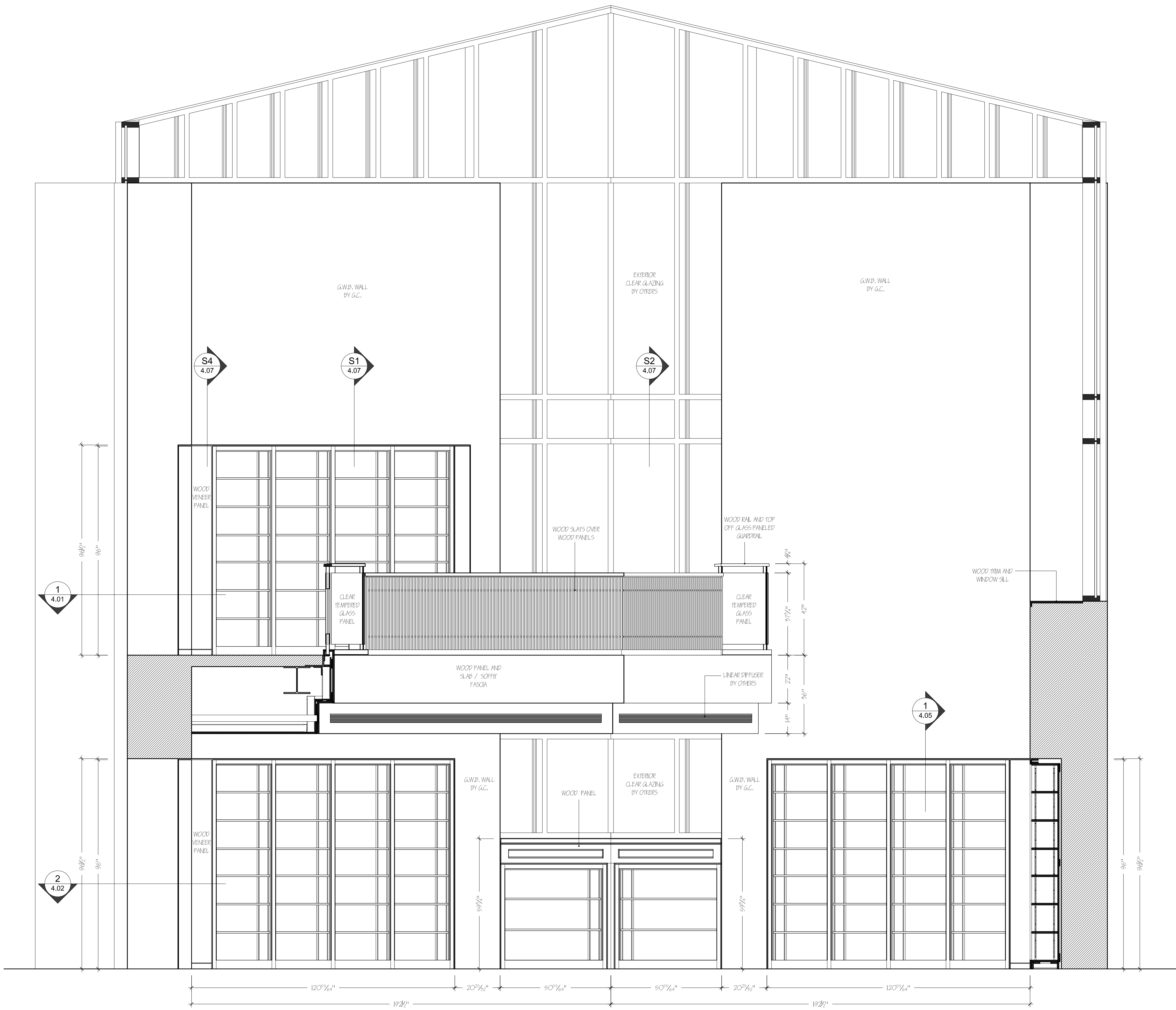
B ELEVATION READING ROOM SCALE: 1/2" = 1'-0"
