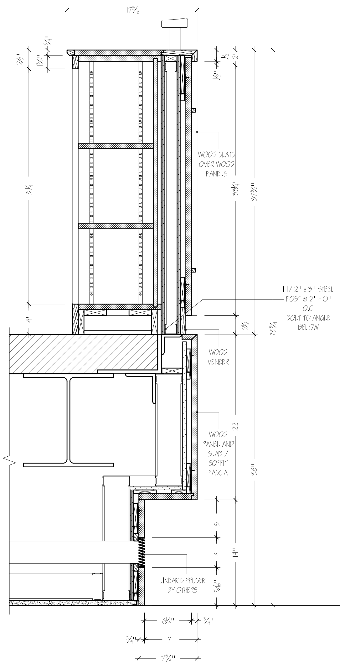
S2 TYPICAL SECTION READING ROOM SCALE: 1-1/2"=1'-0"
