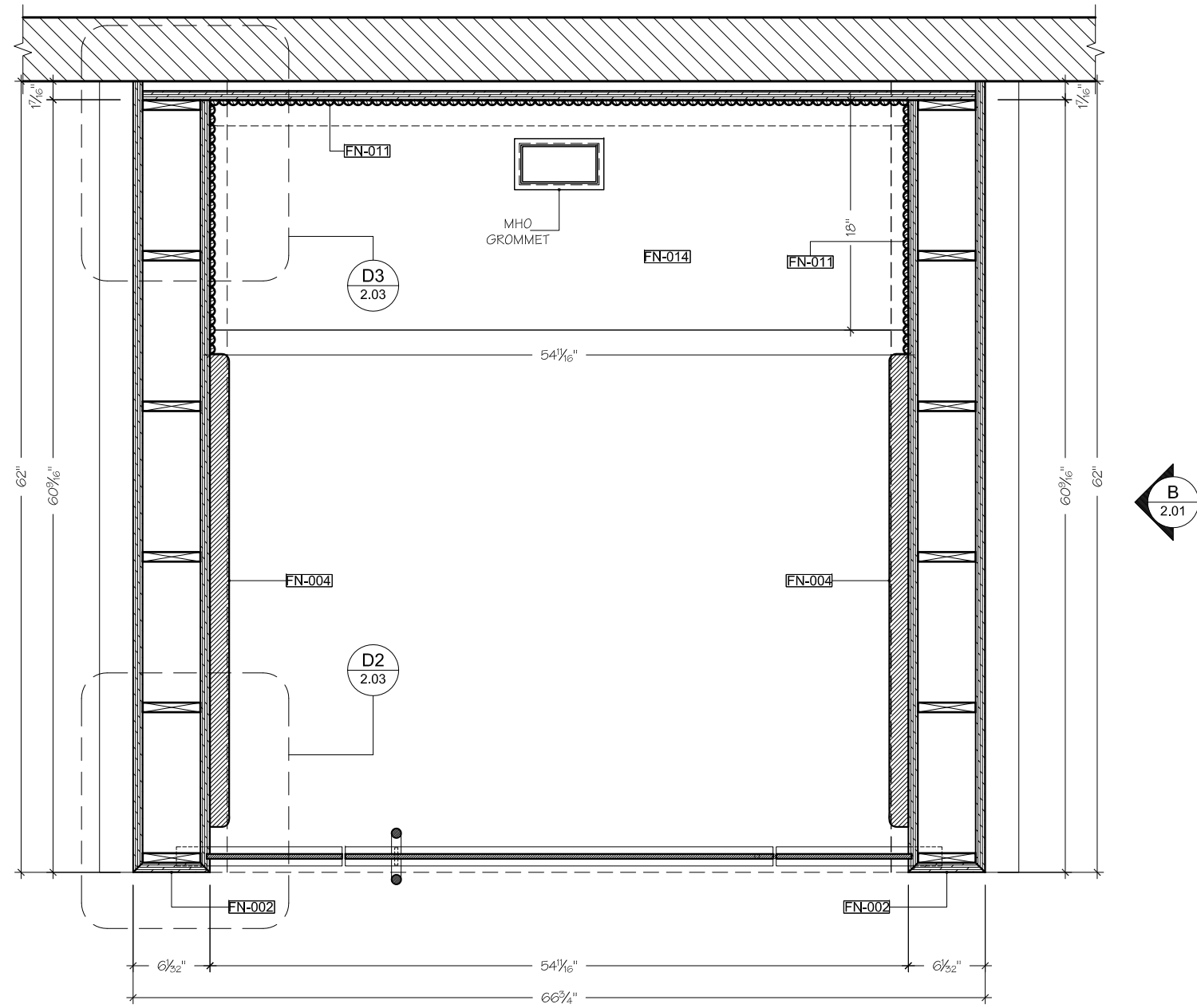
1 PLAN SCALE: 1-1/2" = 1'-0" PHONE BOOTH
