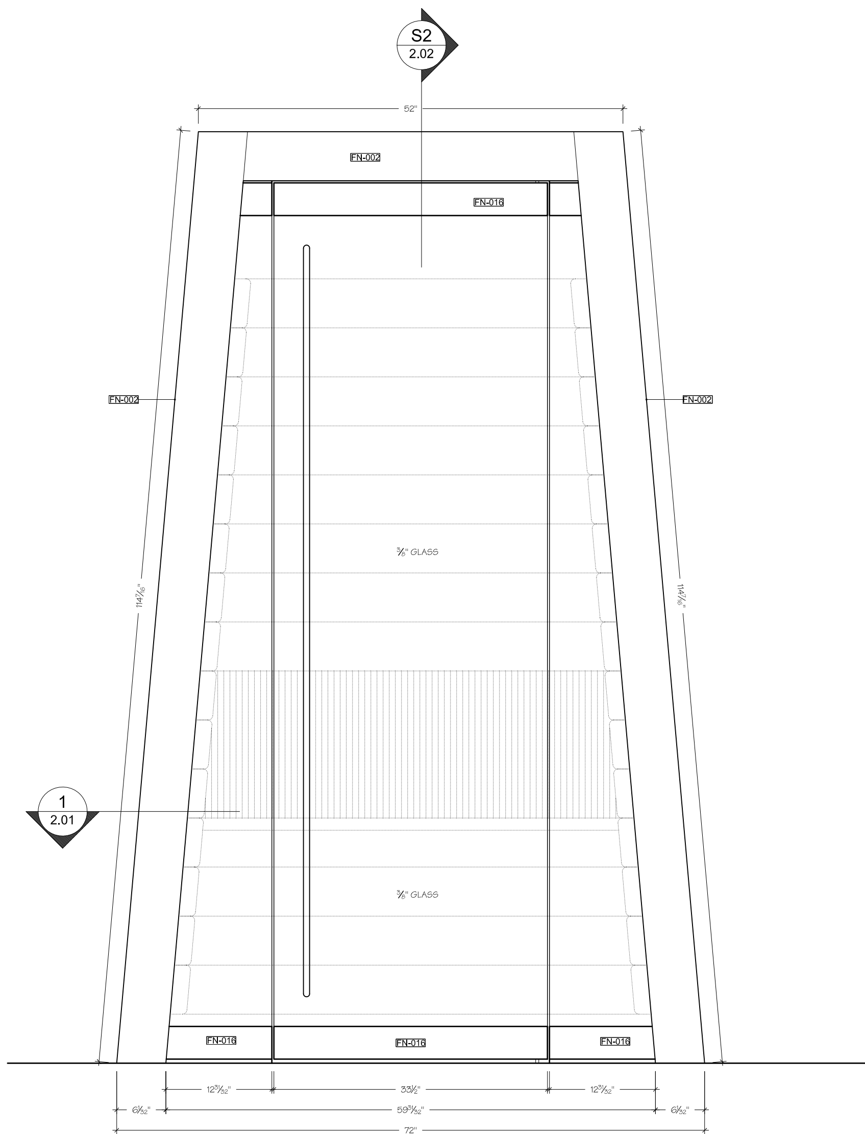
A ELEVATION SCALE: 1-1/2" = 1'-0" PHONE BOOTH
