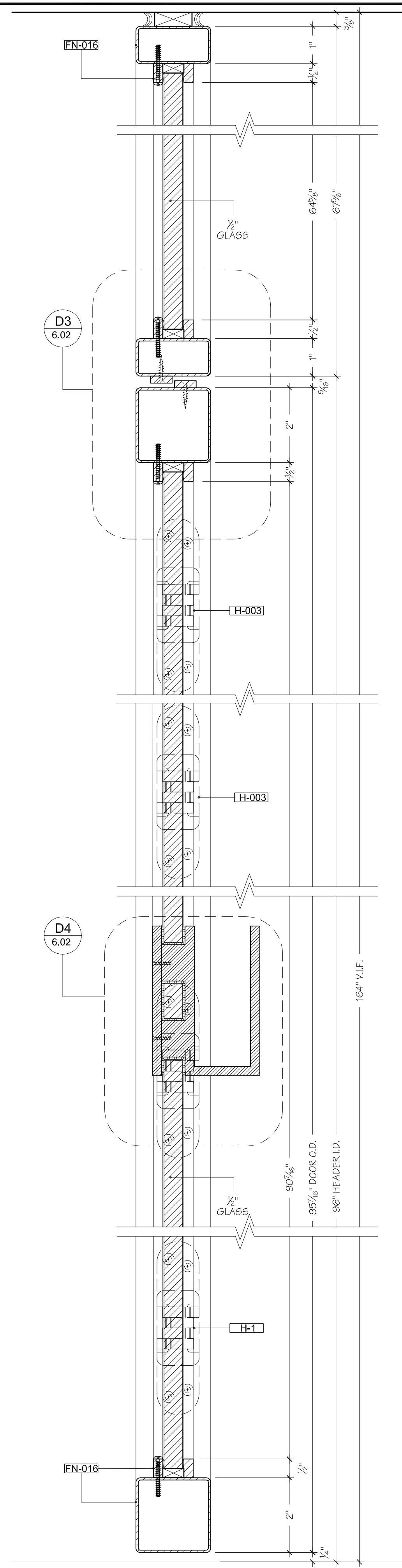
S1 SECTION SCALE: HALF DOOR D04 ELEVATOR LOBBY
