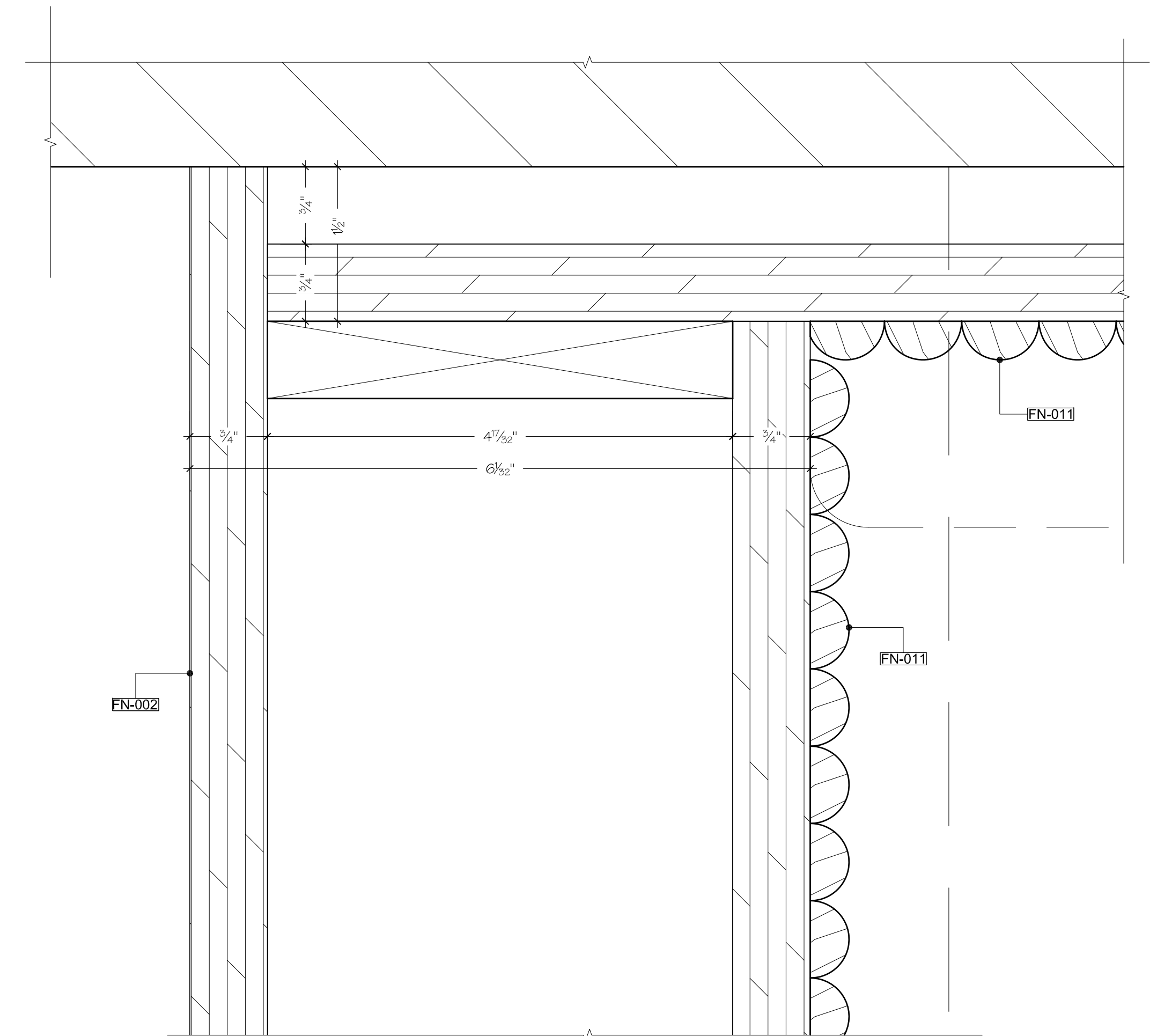
D3 DETAIL SCALE: FULL PHONE BOOTH
