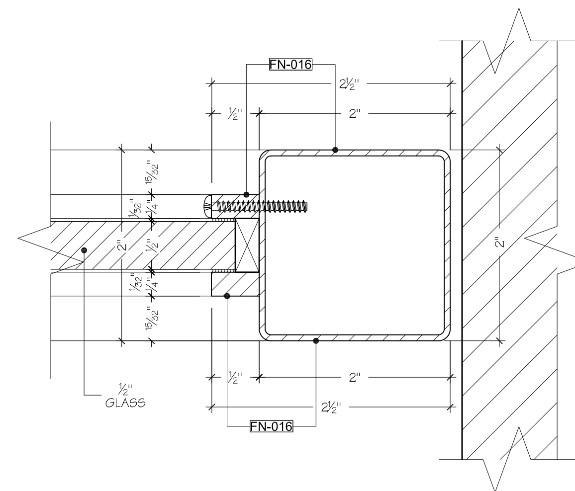
D1 DETAIL SCALE: FULL DOOR D02 WORKING SPACE 01/02
