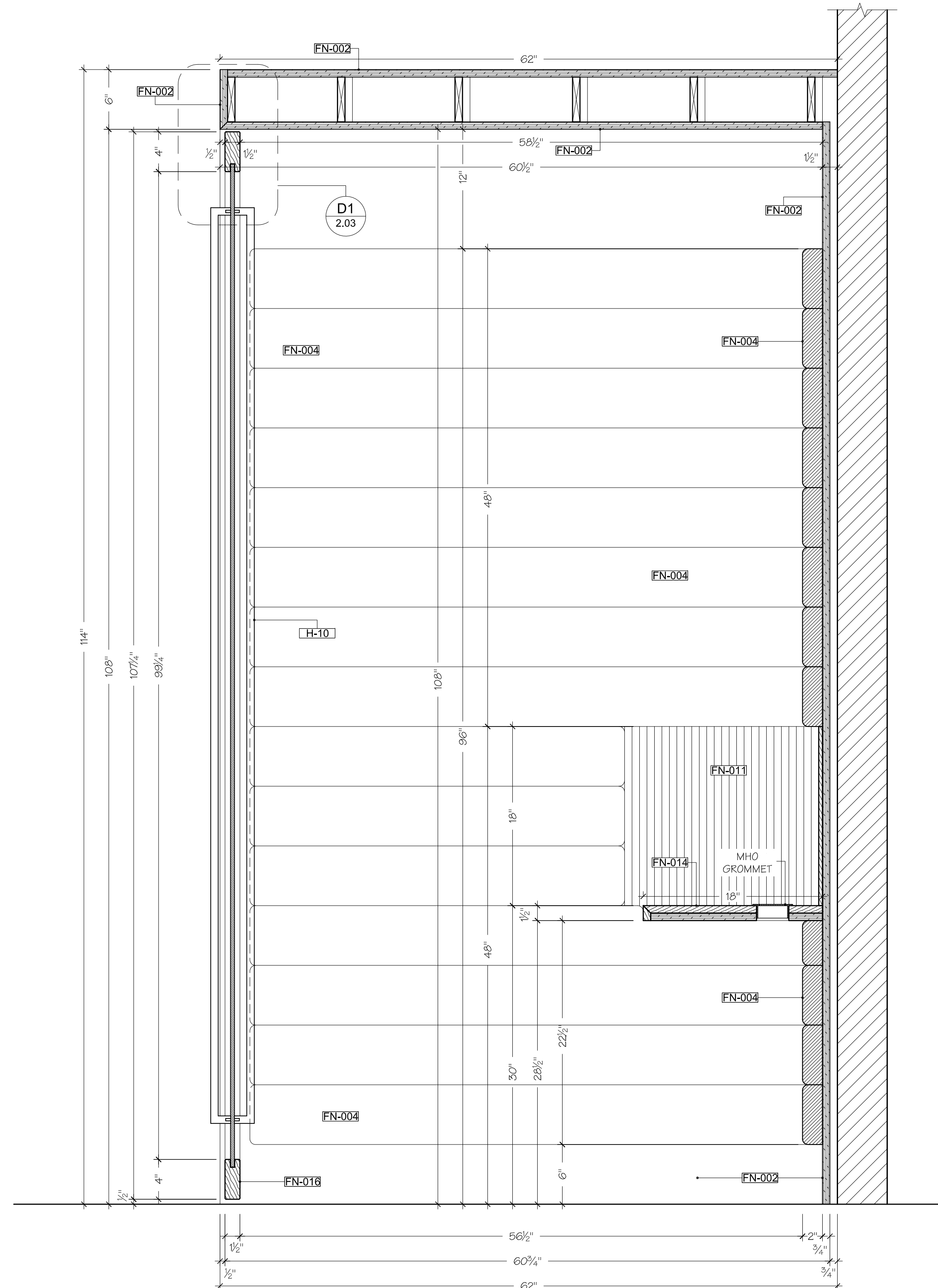
S1 SECTION SCALE: 1-1/2" = 1'- 0" PHONE BOOTH
