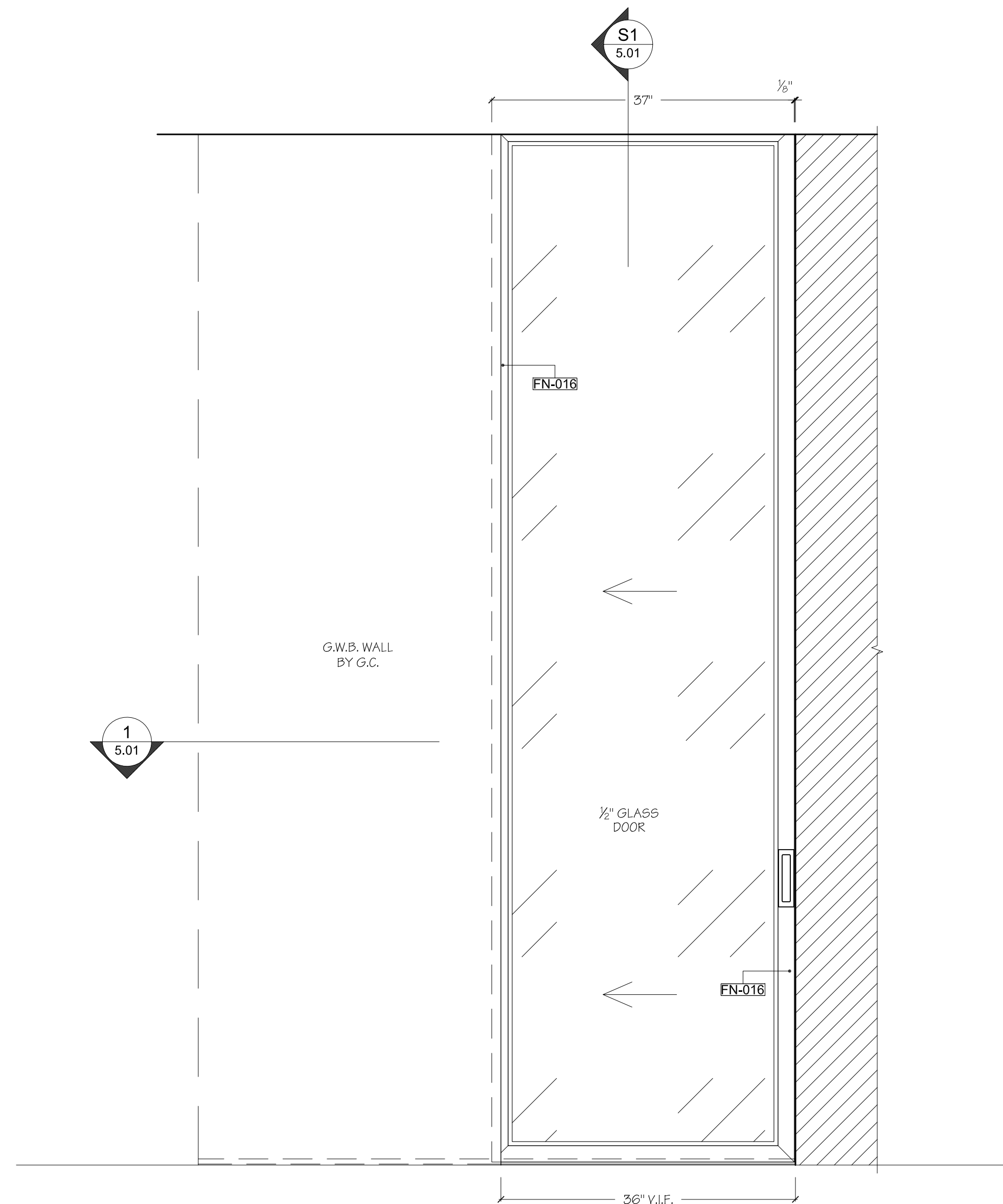
A ELEVATION SCALE: 1" = 1'-0" DOOR D02 WORKING SPACE 01/02
