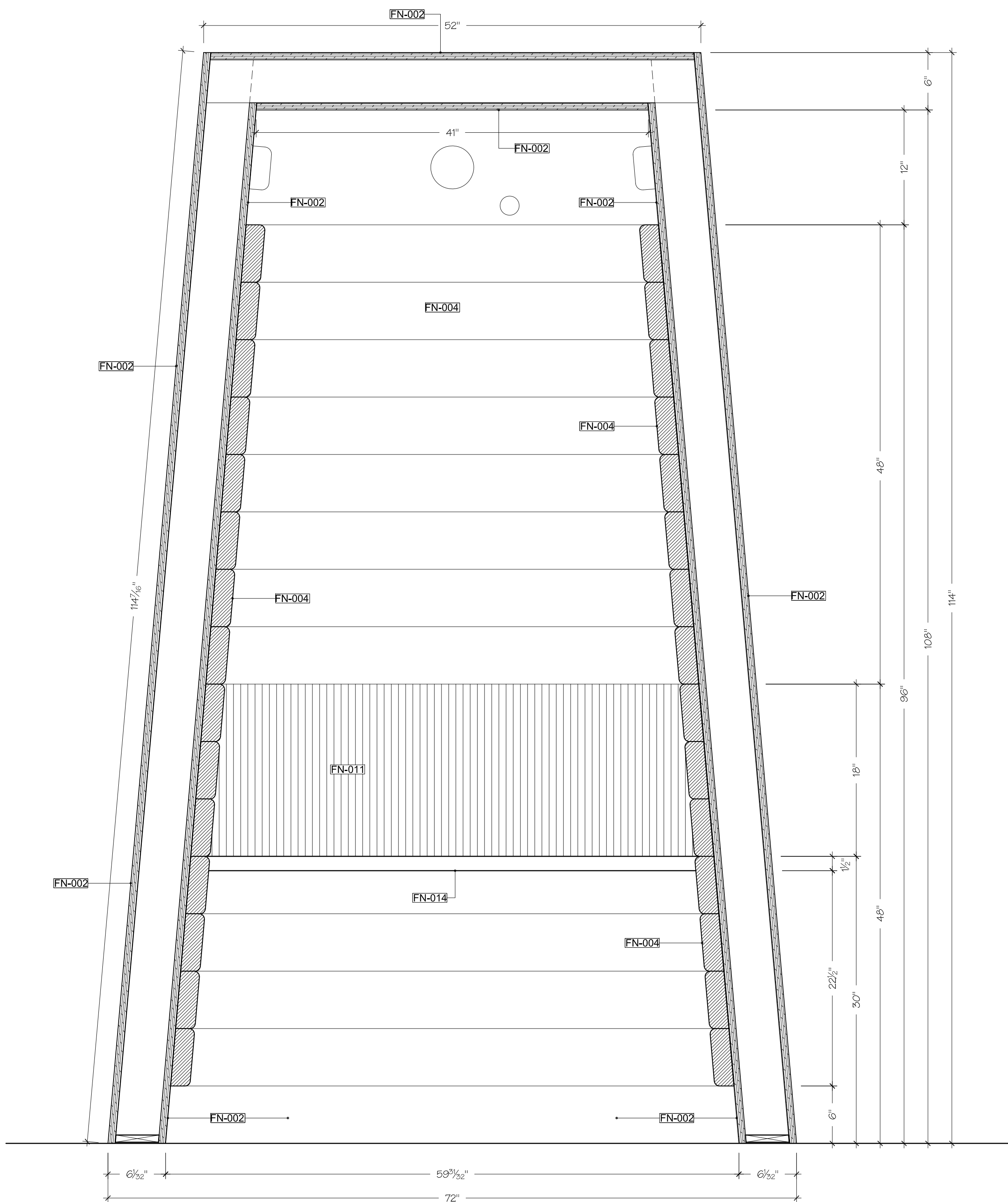
S2 SECTION SCALE: 1-1/2" = 1'- 0" PHONE BOOTH
