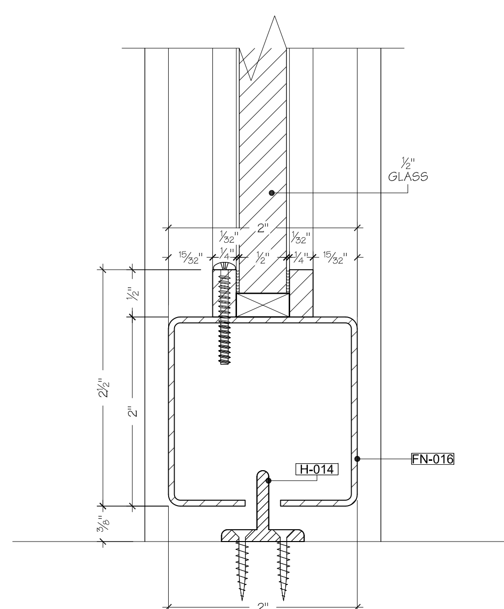
D3 DETAIL SCALE: FULL DOOR D02 WORKING SPACE 01/02
