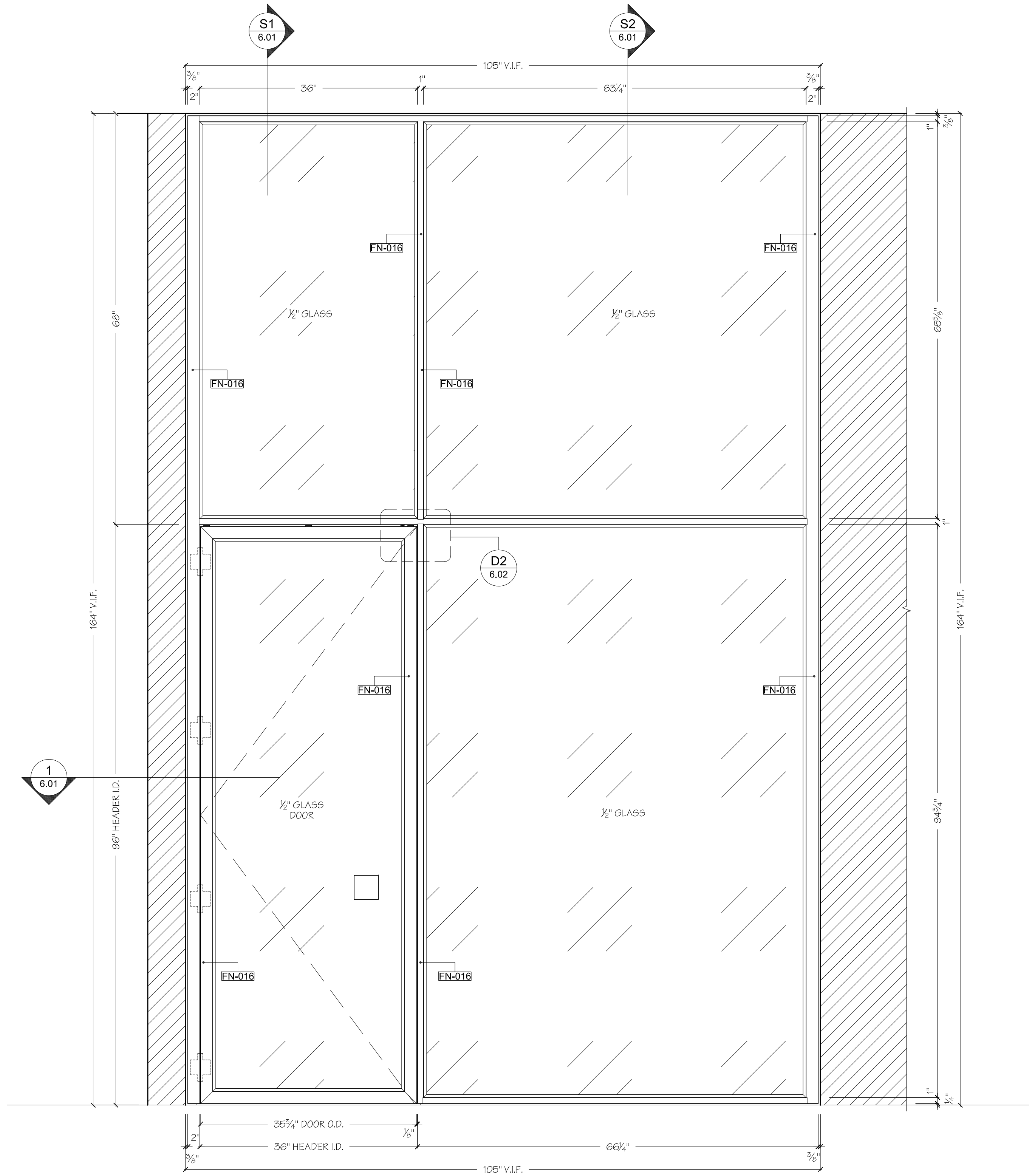
A ELEVATION SCALE: 1" = 1'-0" DOOR D04 ELEVATOR LOBBY
