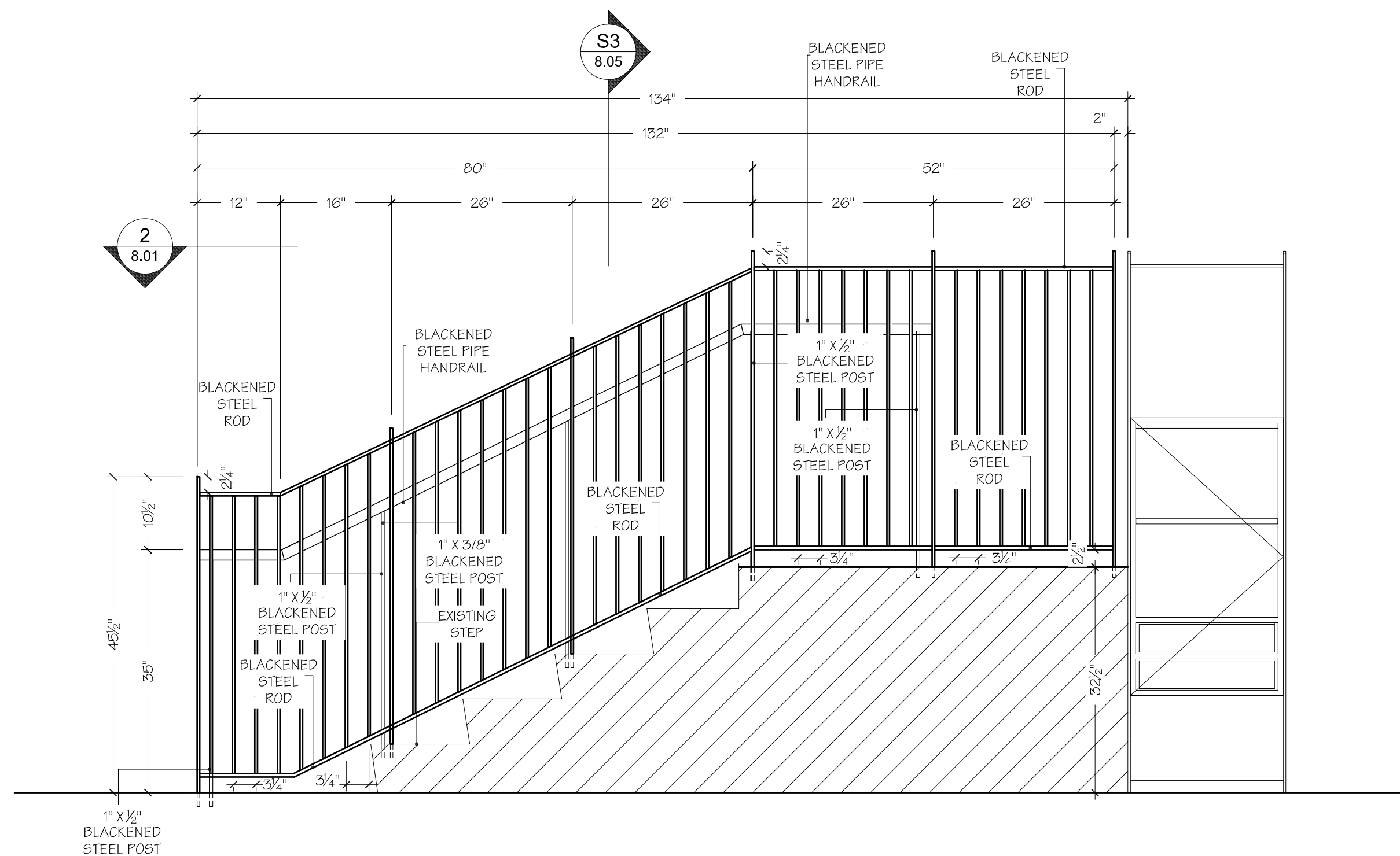
B ELEVATION SCALE: 3/4" = 1'- 0" RAILING
