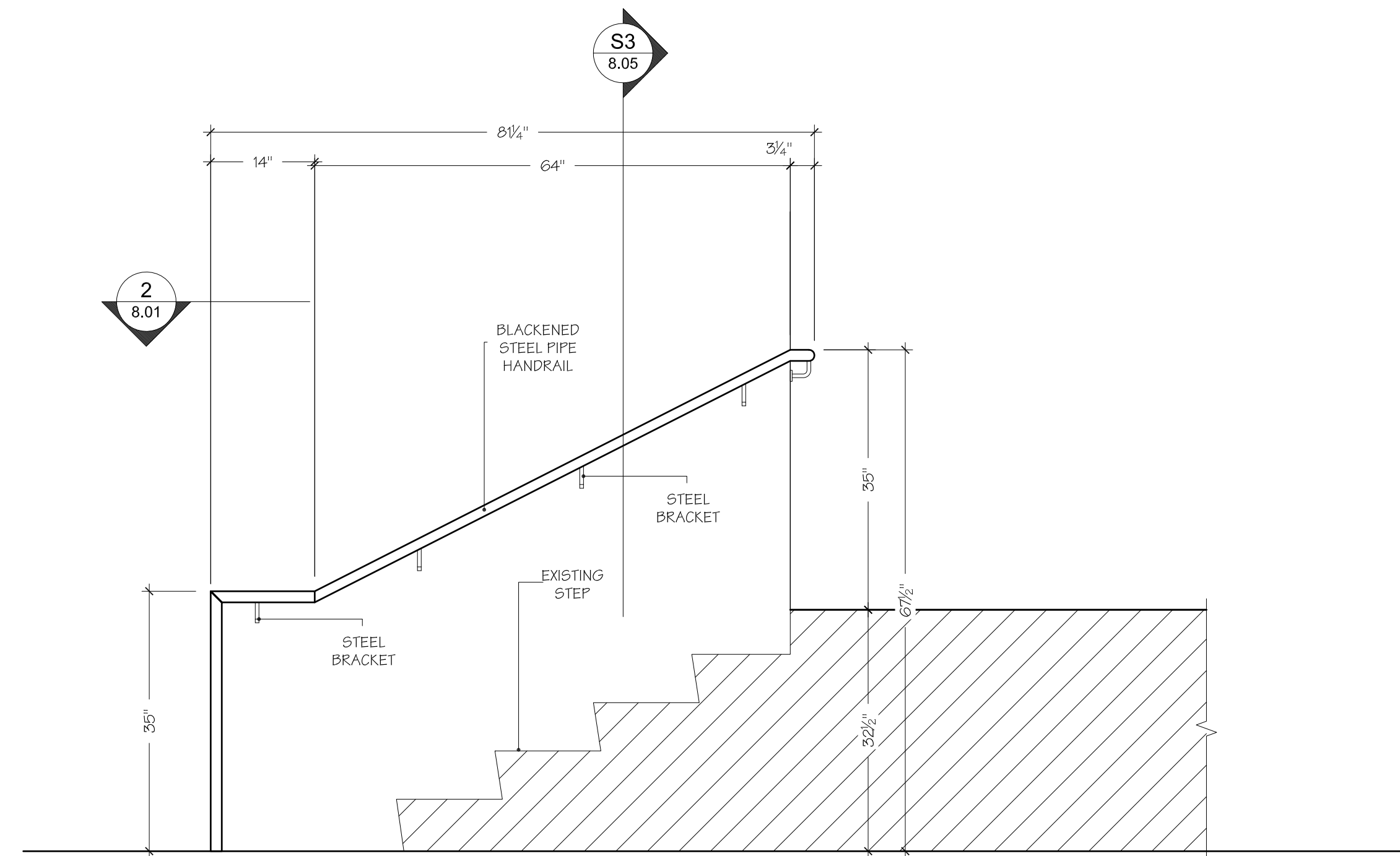
C ELEVATION SCALE: 3/4" = 1'- 0" RAILING
