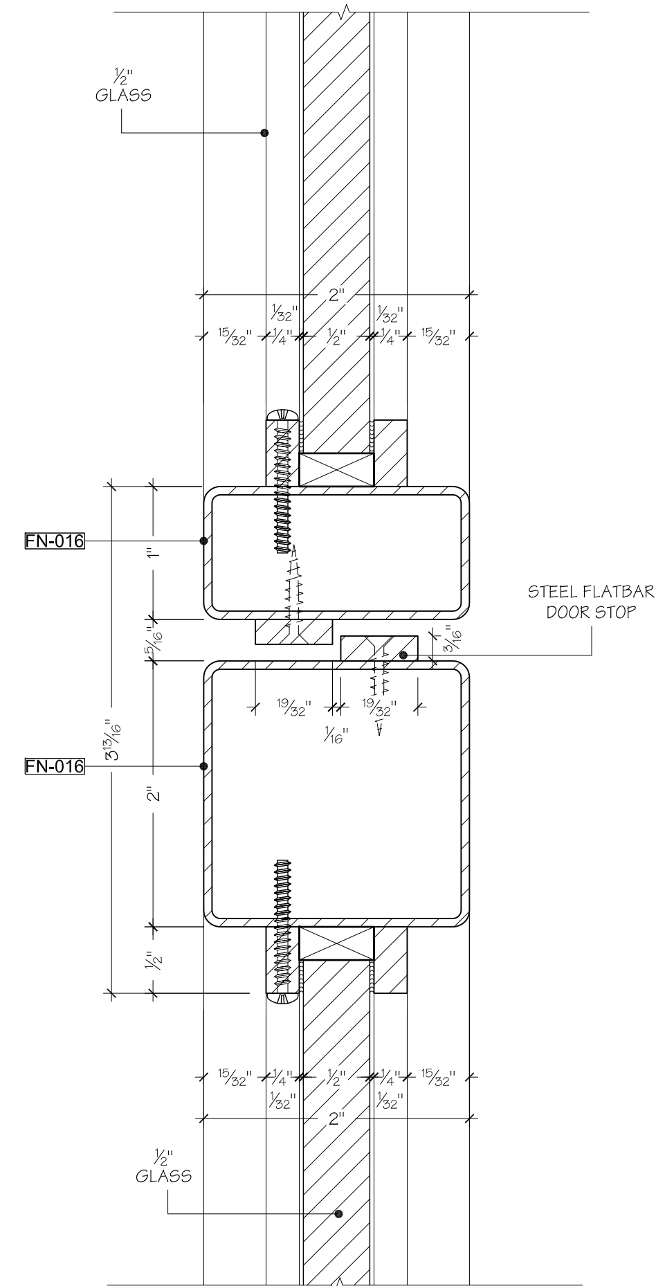
D3 DETAIL SCALE: FULL DOOR D01 ENTRY
