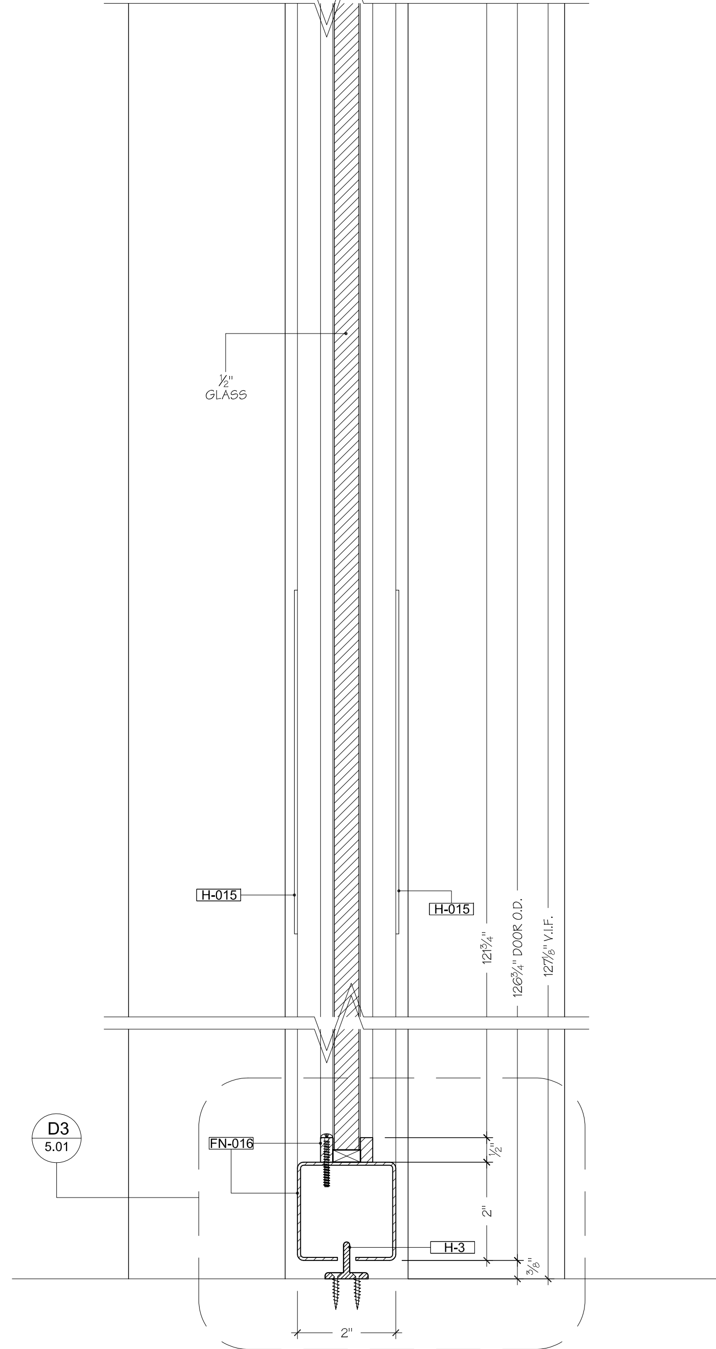
S1 SECTION SCALE: HALF DOOR D02 WORKING SPACE 01/02
